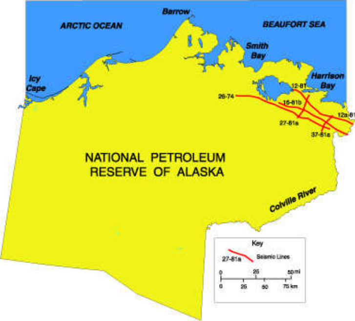
Figure1. Location of Seismic lines used this study
