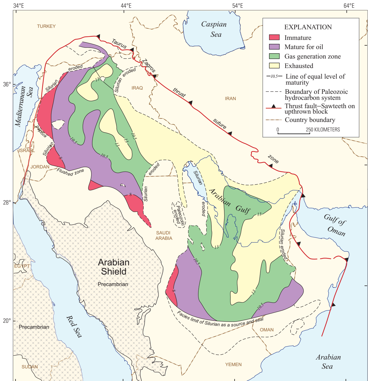
Figure 8. Present-day levels of thermal maturity of Lower Silurian source rock in Arabian Peninsula (modified from Bishop, 1995). Note areas that are currently mature for oil and gas generation in northern Saudi Arabia and western Iraq. Level of maturity (LOM) values shown. Coordinates are approximate.
