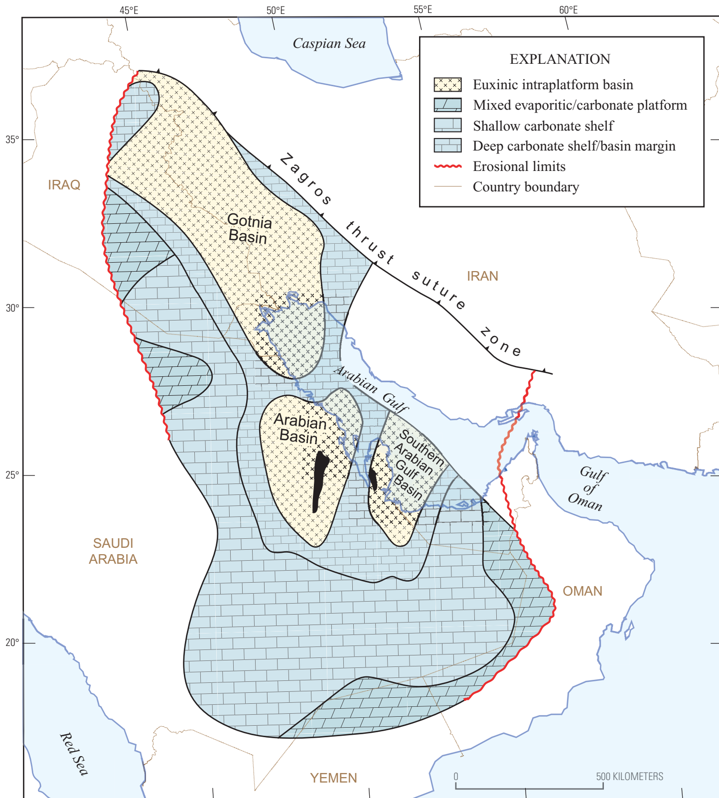
Figure 13. Gotnia, Arabian, and Southern Arabian Gulf Basins in which Jurassic hydrocarbon source rocks accumulated (modified from Alsharhan and Kendall, 1986). Sawteeth on upthrown block of Zagros thrust suture zone.
