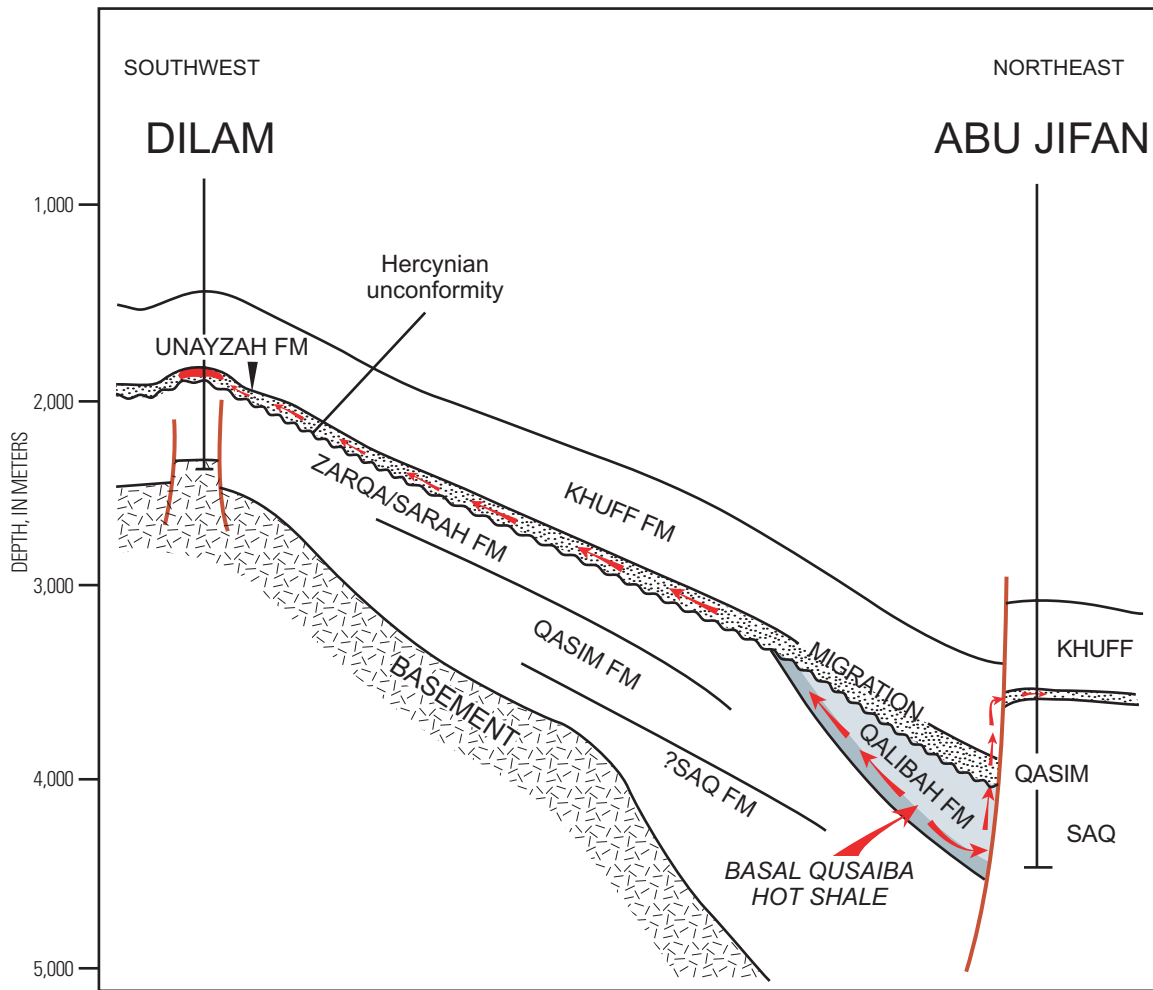
Figure 10. Diagrammatic model for migration of hydrocarbons generated from basal Qusaiba “hot shale” in central Saudi Arabia (modified from McGillivray and Al-Husseini, 1992). Note that petroleum (red) migrates upward to the Hercynian unconformity (wavy line) and laterally into the Unayzah Formation, which acts as the conduit for updip migration. This model may be applicable to a similar situation in the Widyan Basin to the north.
