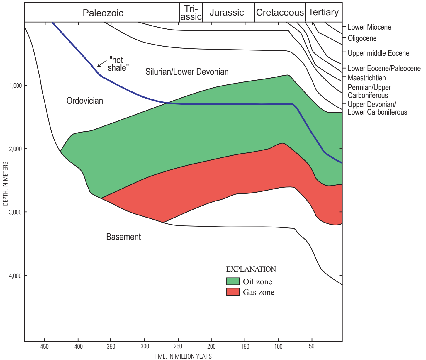
Figure 9. Burial history model of Akkas-1 well of western Iraq (modified from Agrawi, 1998). Basal Silurian “hot shale” source rock is shown to have remained in the oil generation window since the late Paleozoic. Location of the Akkas-1 well shown in figure 3.
