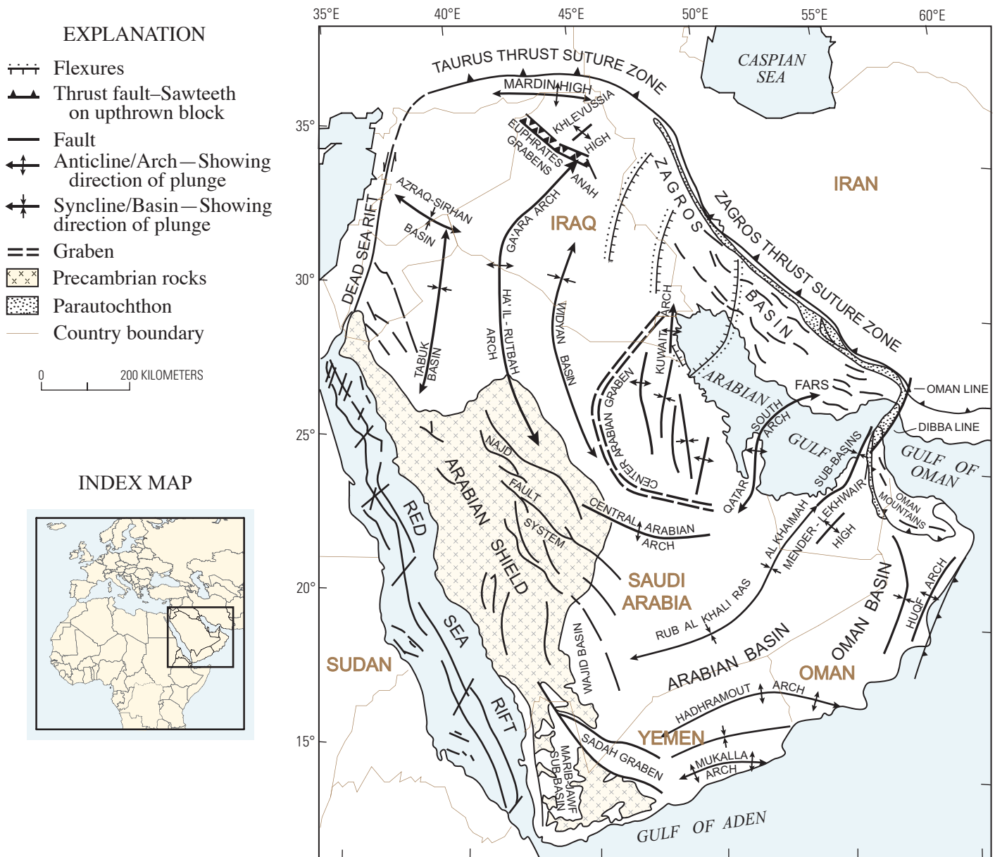
Figure 1. Structural provinces of Arabian Peninsula (modified from Al-Laboun, 1986). Coordinates are approximate.
