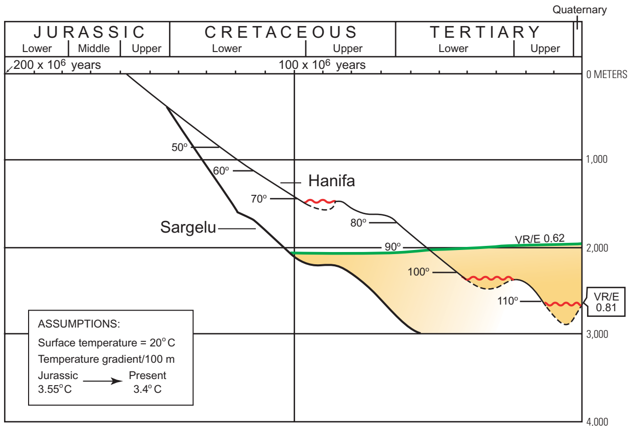
Figure 15. Burial history of the Hanifa and Sargelu Formations (modified from Murris, 1981). Mature zone is colored yellow. VR/E, calculated maturity in vitrinite reflectance equivalent units. Periods of uplift and erosion shown (dashed line); corrected burial history curve shown (wavy red line).
