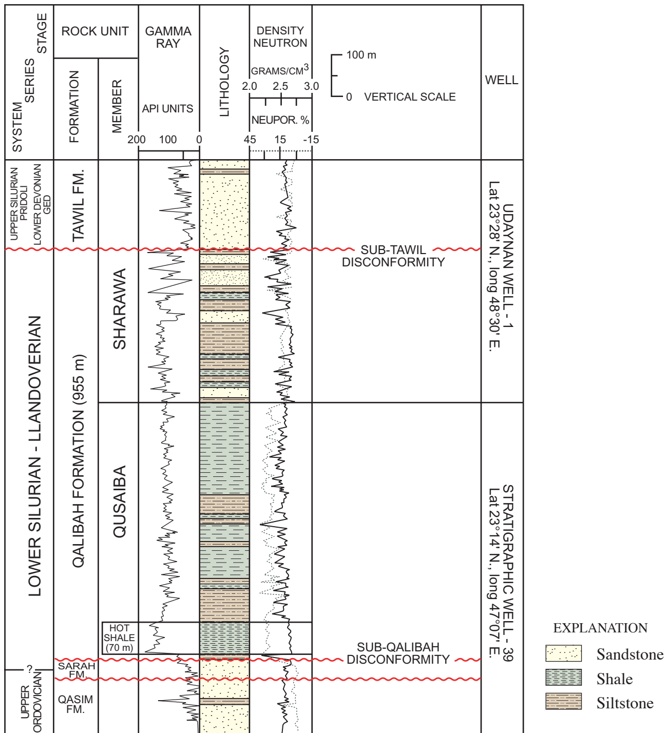
Figure 6. Subsurface composite reference section for the Qalibah Formation in central Saudi Arabia, showing lithology, biostratigraphy, and gamma ray-density-neutron well-log patterns (modified from Mahmoud and others, 1992). Note “hot shale” unit of basal Qusaiba Member. NEUPOR. %, neutron log porosity in percent.
